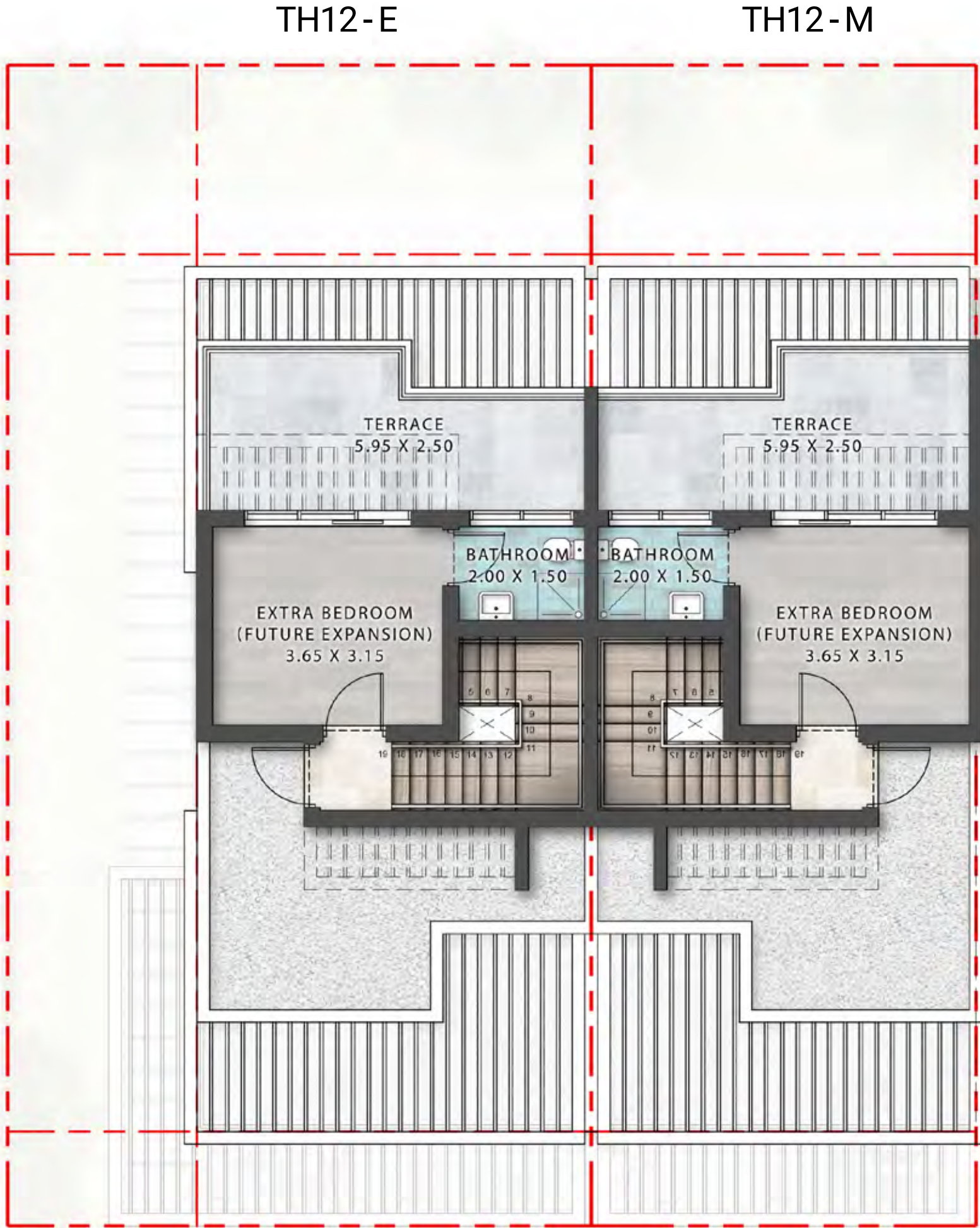
ROOF FLOOR (FUTURE EXPANSION)
