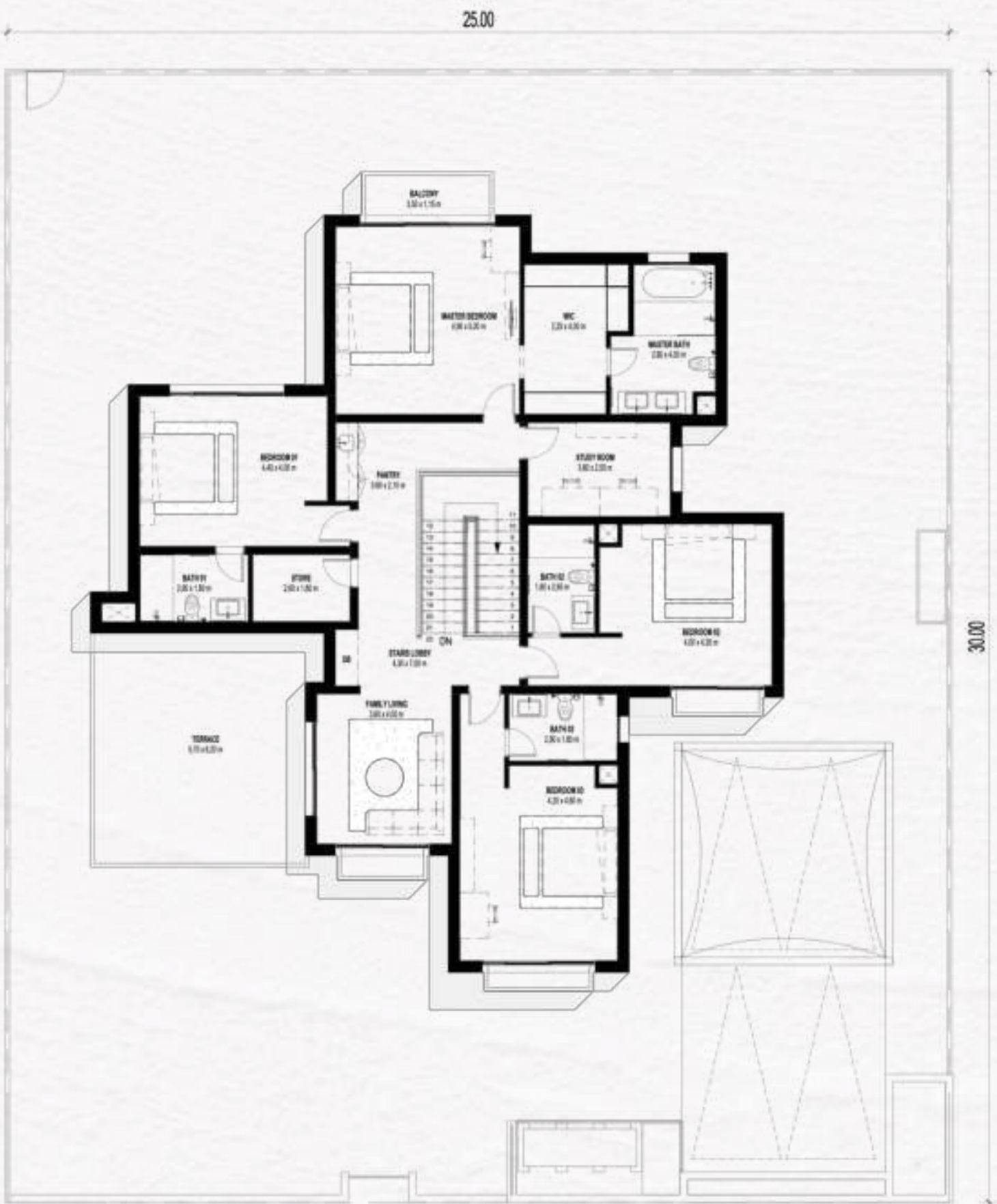
FIRST FLOOR
