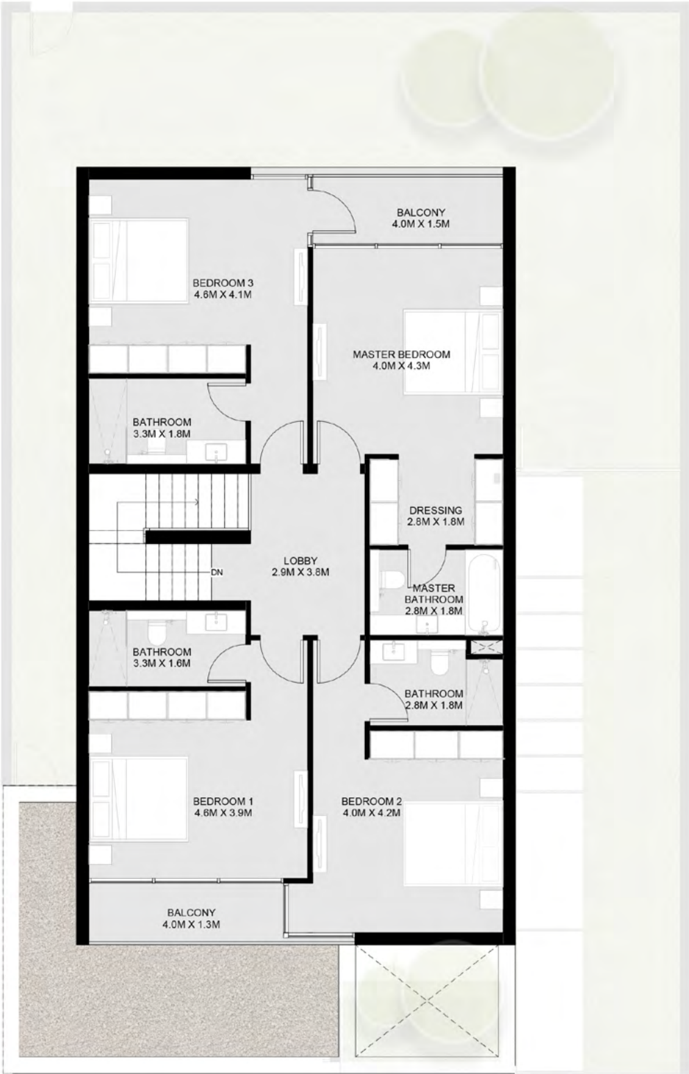
First Floor
