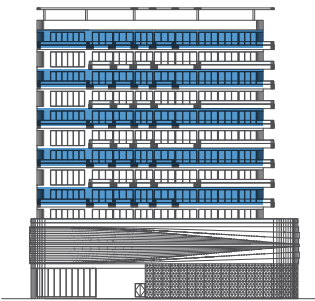
ELEVATION C
