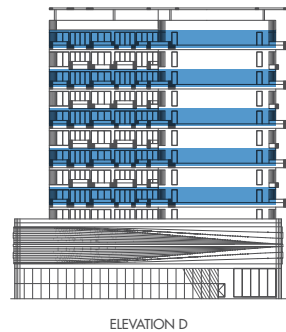
ELEVATION D
