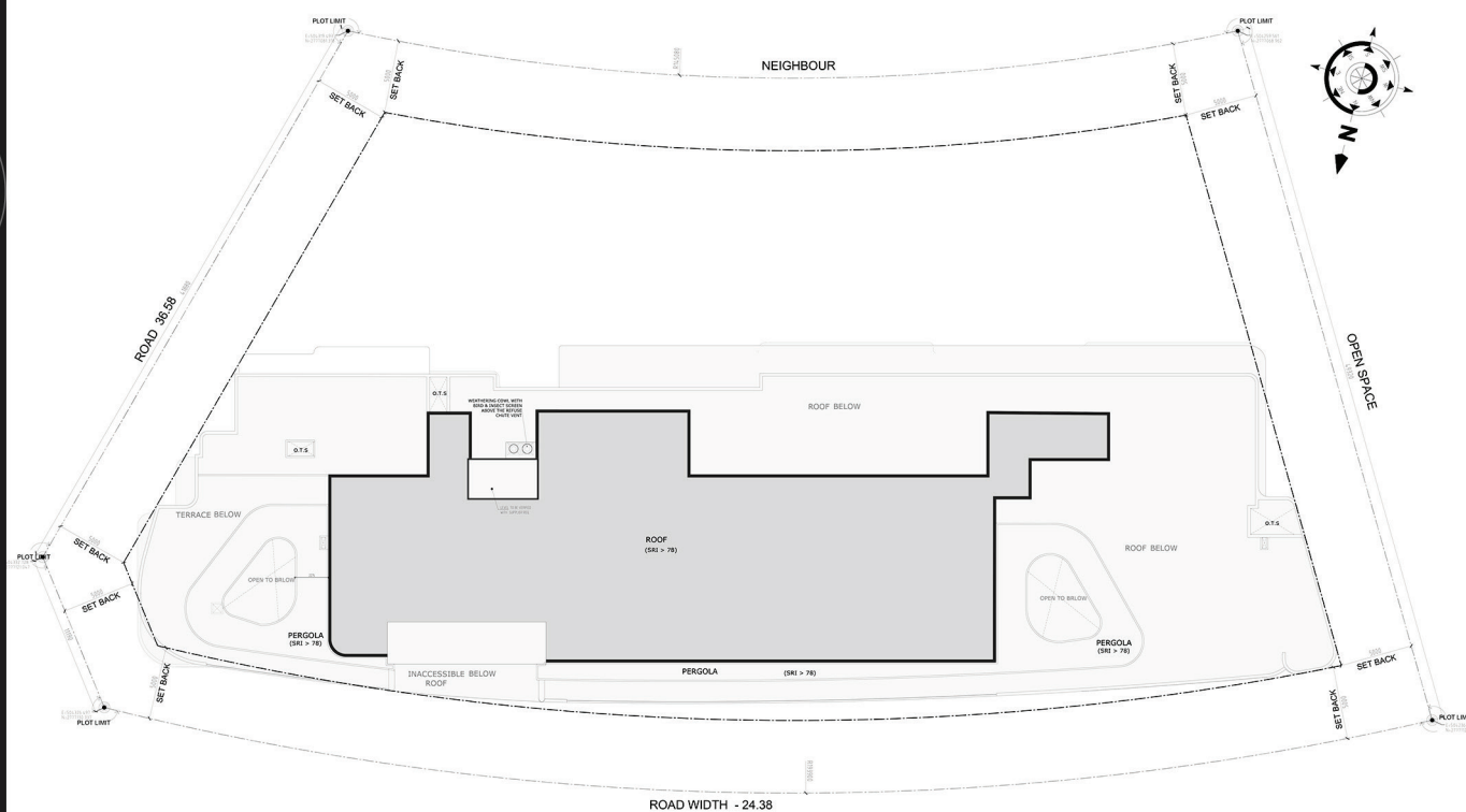
UPPER ROOF PLAN
