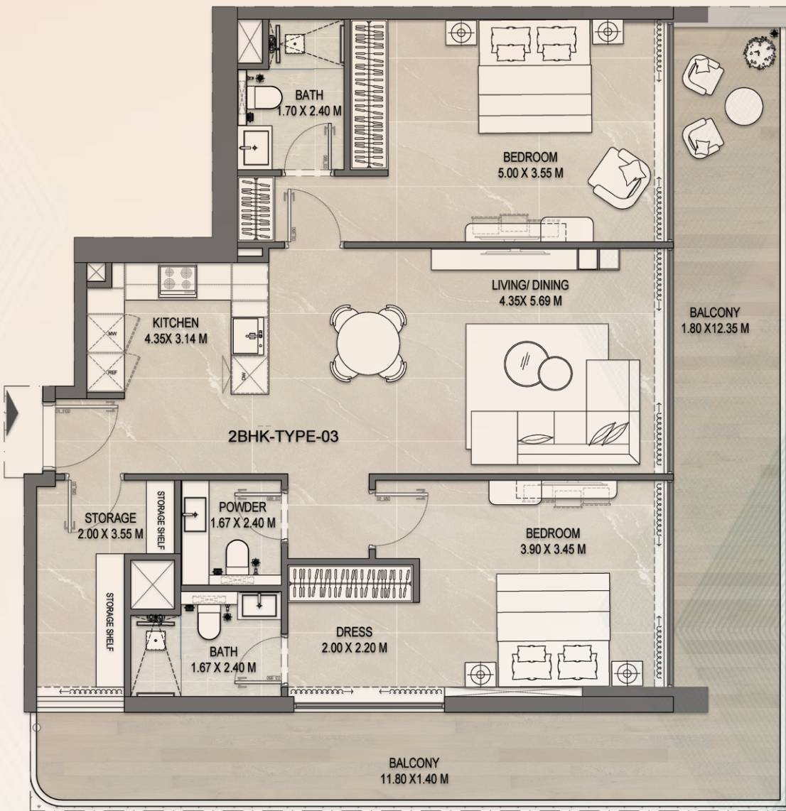
01 2BHK TYPE-03 FURNITURE PLAN SCALE 1:100@A1
