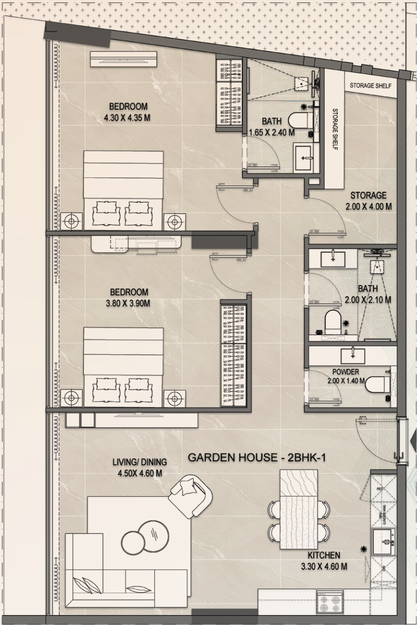
01 GARDEN HOUSE 2BHK-1 SCALE 1:100@A1
