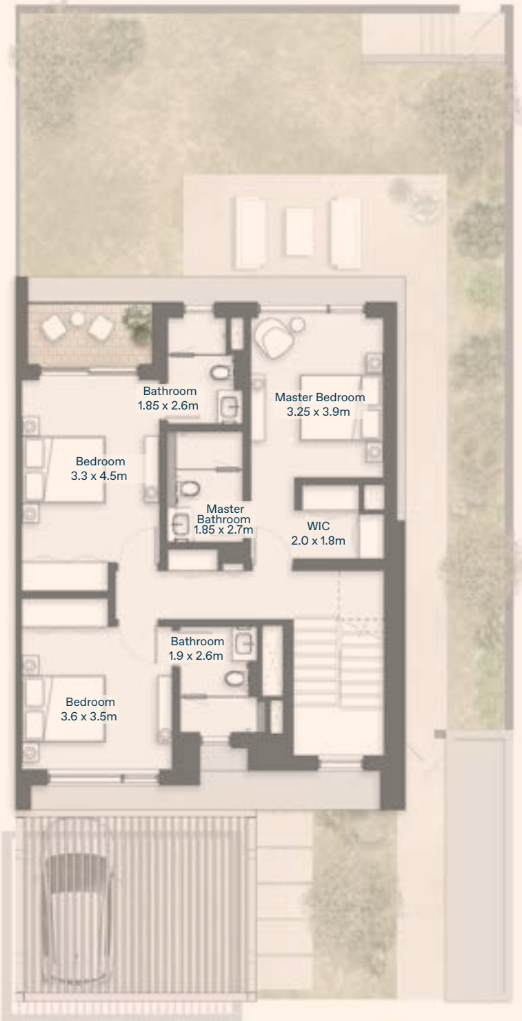
First Floor
