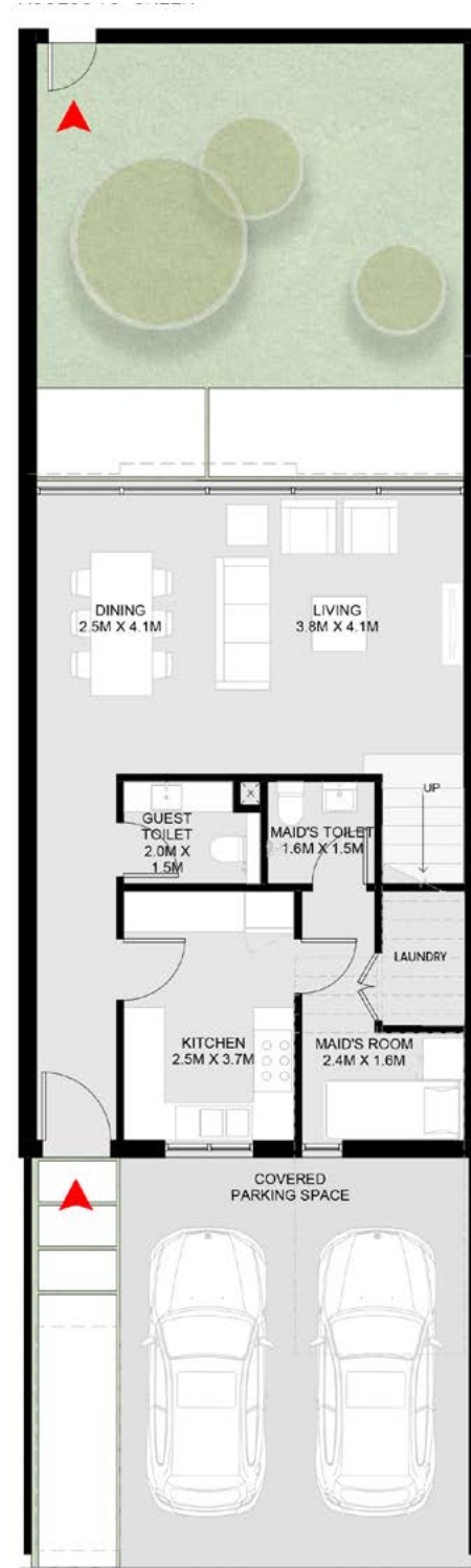
Ground Floor
